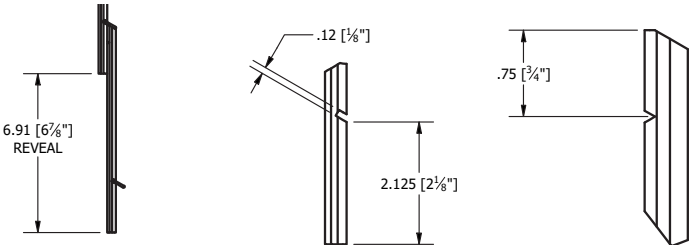
STACKED VIEW SCALE 1 / 5
