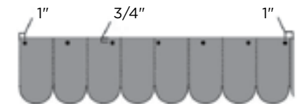
Nail Placement 8" o.c. Detail Figure 6c
